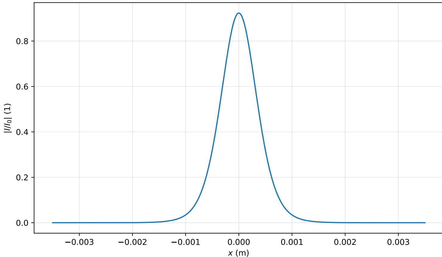
Intensity profile I(x, y = 0, z = 2.070m)/I_0 , P_{in}=0.6P_{cr} , artificial time
